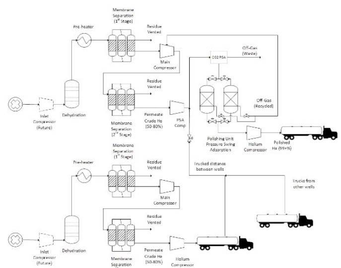
The production process for Helium
